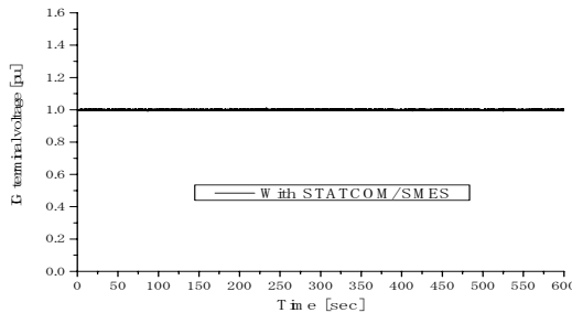
Fig 10. Response of IG terminal voltage
