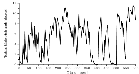
Fig 7. Blade pitch angle of wind turbine
