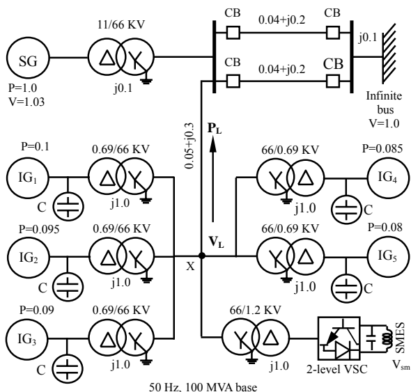
Fig 1. Power system model with STATCOM/SMES
