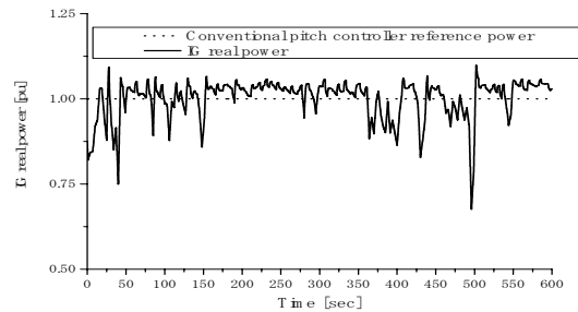
Fig 5. Real power of IG with only conventional pitch controller
