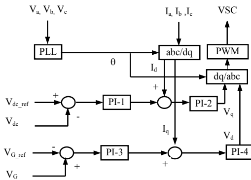
Fig 3. Control system of the VSC
