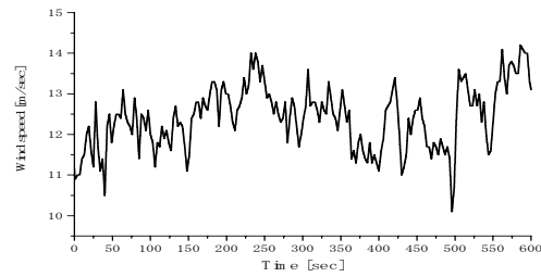
Fig 4. Response of real wind data
