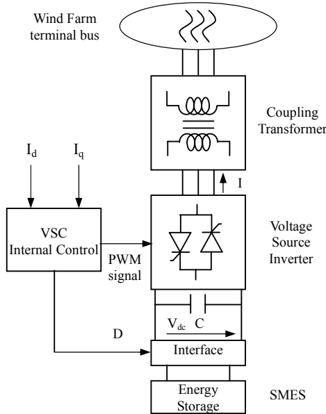
Fig 2. Configuration of STATCOM/SMES topology
